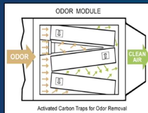
Odor Control Media Bed (optional)
